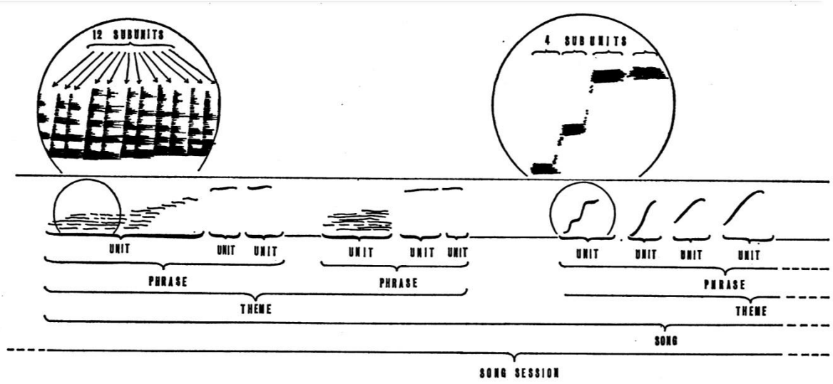
Fig. 1. Diagrammatic sample of whale spectrograms (also called sonagrams) indicating terminology used in describing songs. Frequency is given on the vertical axis, time on the horizontal axis. The circled areas are spectrograms that have been enlarged to show the substructure of sounds which, unless slowed down, are not readily detected by the human ear.
